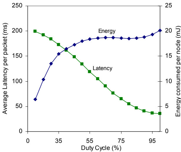
Fig.2 Latency and energy consumption results of SMAC obtained from queueing modeling
