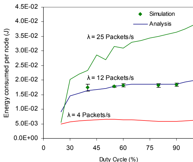
Fig.4 Energy consumption results for SMAC obtained from queuing analysis and simulation
