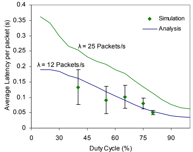
Fig.3 Latency results for SMAC obtained from queueing analysis and simulation
